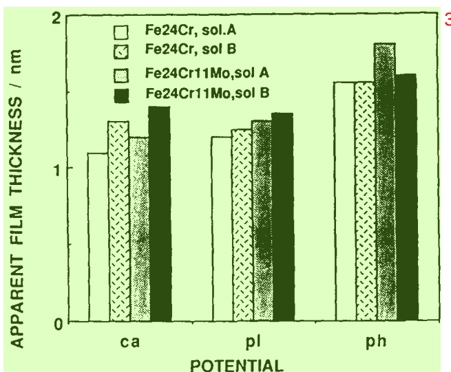
Fig.6 Apparent Film Thickness Calculated from Cr 2p 3/2 XPS Peaks 4
