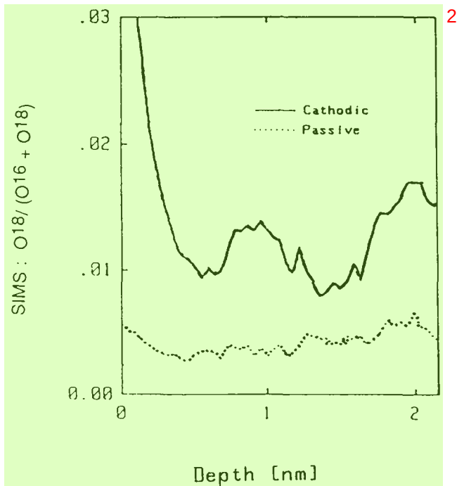
Fig. 5 SIMS Intensity Ratio ^{18}\text{O}/^{16}\text{O} + ^{18}\text{O} for Fe 24 Cr Polarised in Electrolyte (A) at Potentials CA and PH
