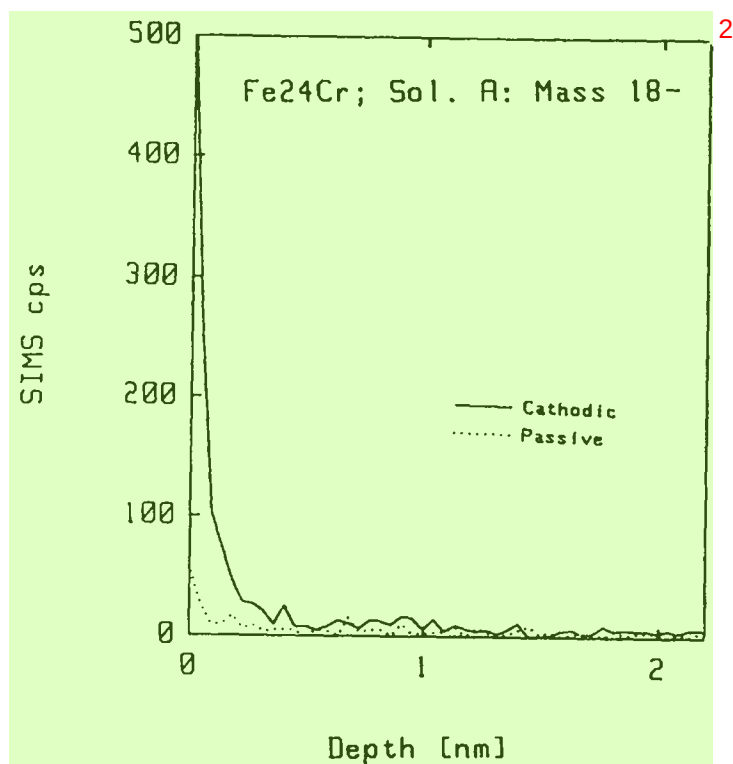
Fig.4 SIMS Depth Profile of ^{18}\text{O} on Fe24Cr Alloy Polarised at Potentials CA and PH in Electrolyte (A)
