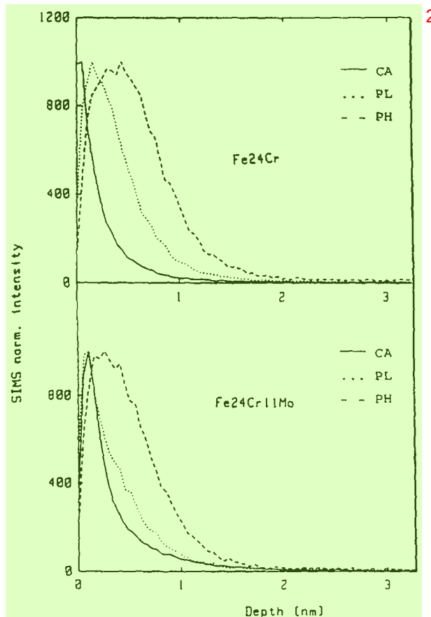
Fig.8 Normalised SIMS Cl - Profiles measured on Fe 24 Cr and Fe 24 Cr 11 Mo polarised at CA, PL, and PH. 3
